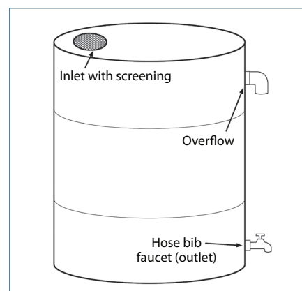
Figure 2. Diagram of rain barrel components.
